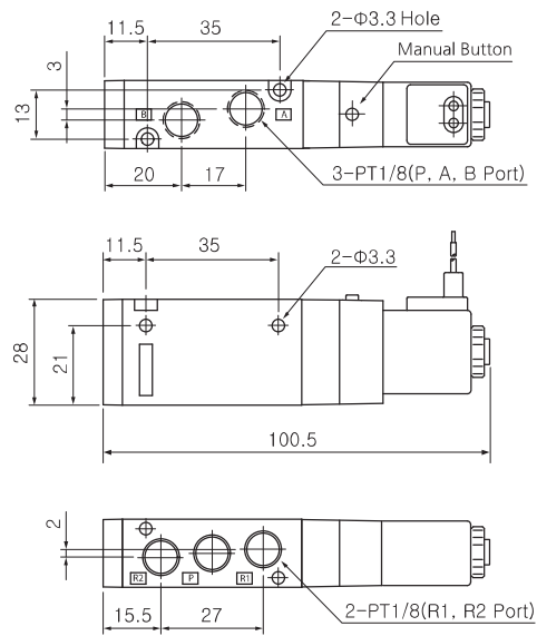
2position / 5port single(Grommet type)
