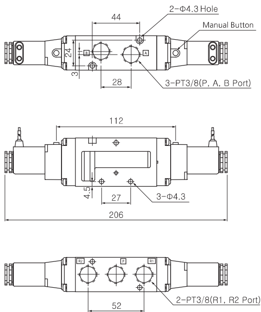
2position / 5port double(Grommet type)
