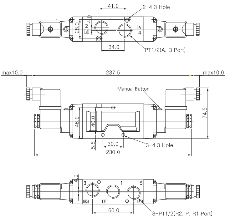
2position / 5port double(Connector type)
