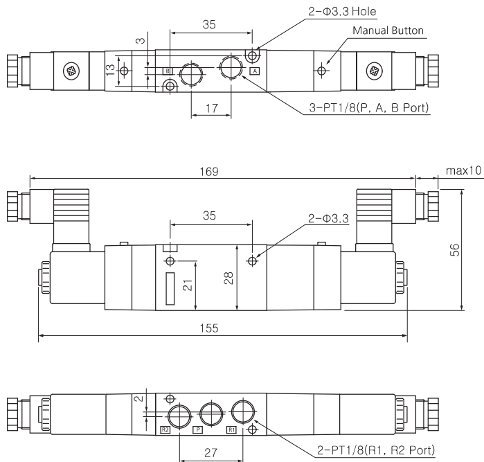
3position / 5port double (Connector type)
