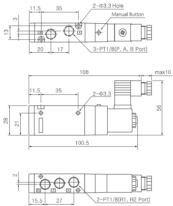
2position / 5port single(Connector type)
