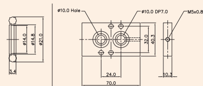
Single Acting Use Plate SN3000-Plate
