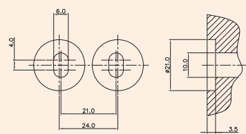
Sealing Area
